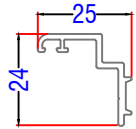
3746 - Swing Door Rebate (Adjustable Jamb)
